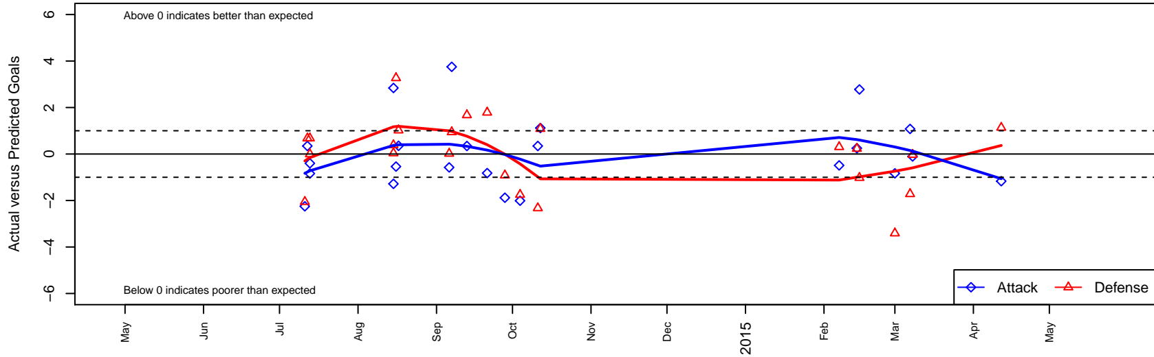
PCU White B00 Dots are actual minus expected GF (blue circles) and GA (red triangles). Blue line is smoothed change in attack strength. Red is smoothed change in defense strength.
